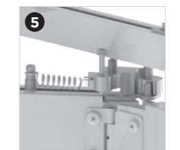
Ensemble de cames de compression
